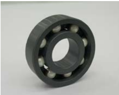
Full Ceramic Bearing Silicon nitride inner and outer ring. Silicon nitride rolling element. Zirconia ball.
